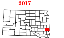
UNIVERSAL TRANSVERSE MERCATOR PROJECTION
