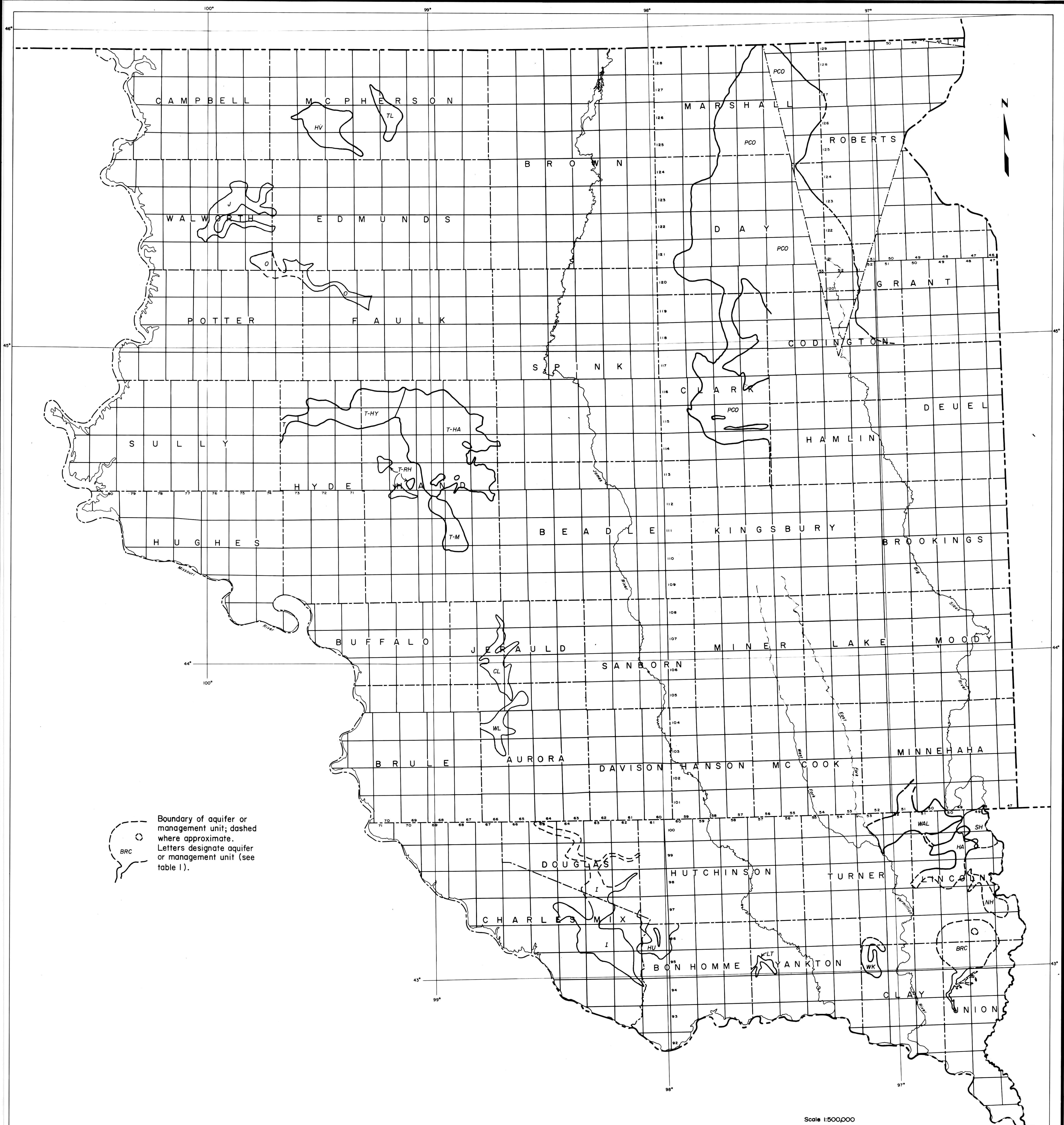
PLATE 6 MAP OF EASTERN SOUTH DAKOTA SHOWING LOCATION OF THE INTERMEDIATE AQUIFER SYSTEM
