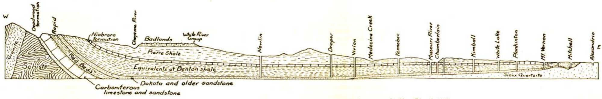
Section across central South Dakota from the Sioux quartzite region to the Black Hills. After Darton
