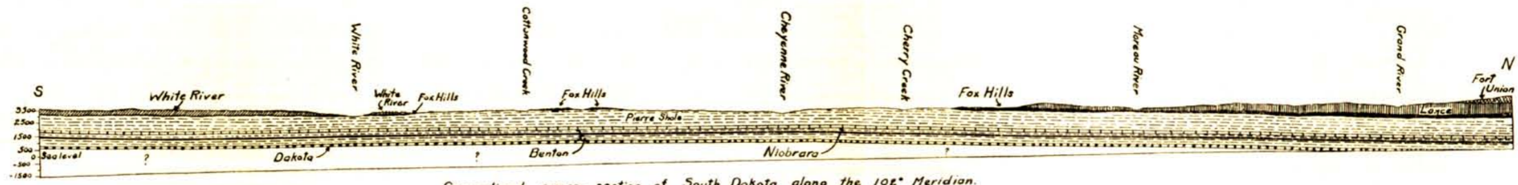
Generalized cross-section of South Dakota along the 102° Meridian. (Altitude of the Dakota sandstone modified after Darton)
