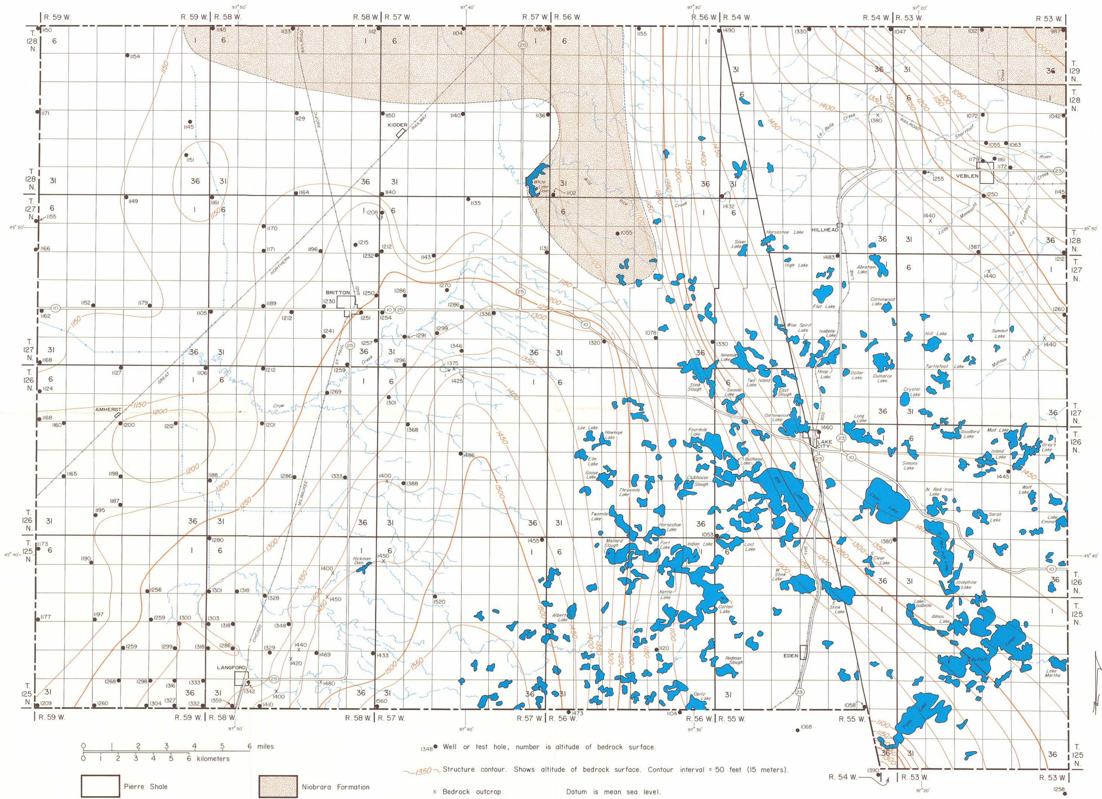
Plate I. Structure contour map of the bedrock surface.
