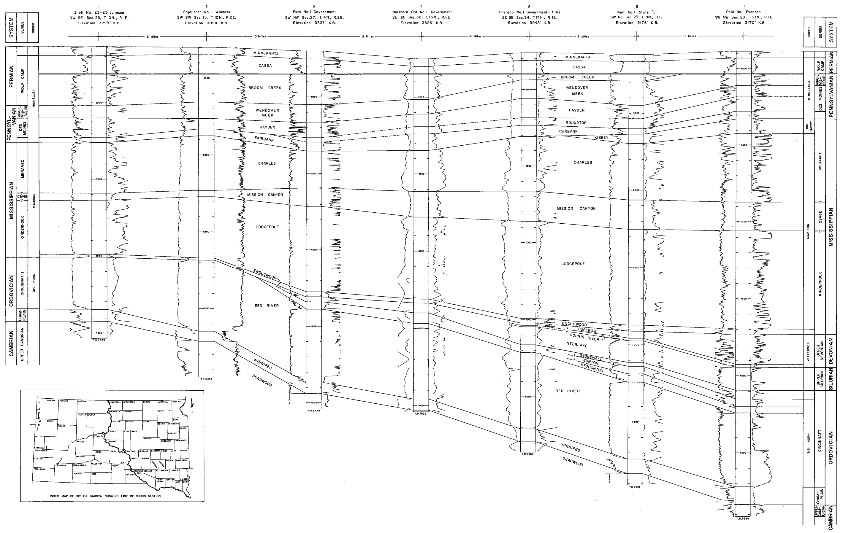
Figure 10. North-South Cross Section of Paleozoic Rocks of Western Butte and Harding Counties.
