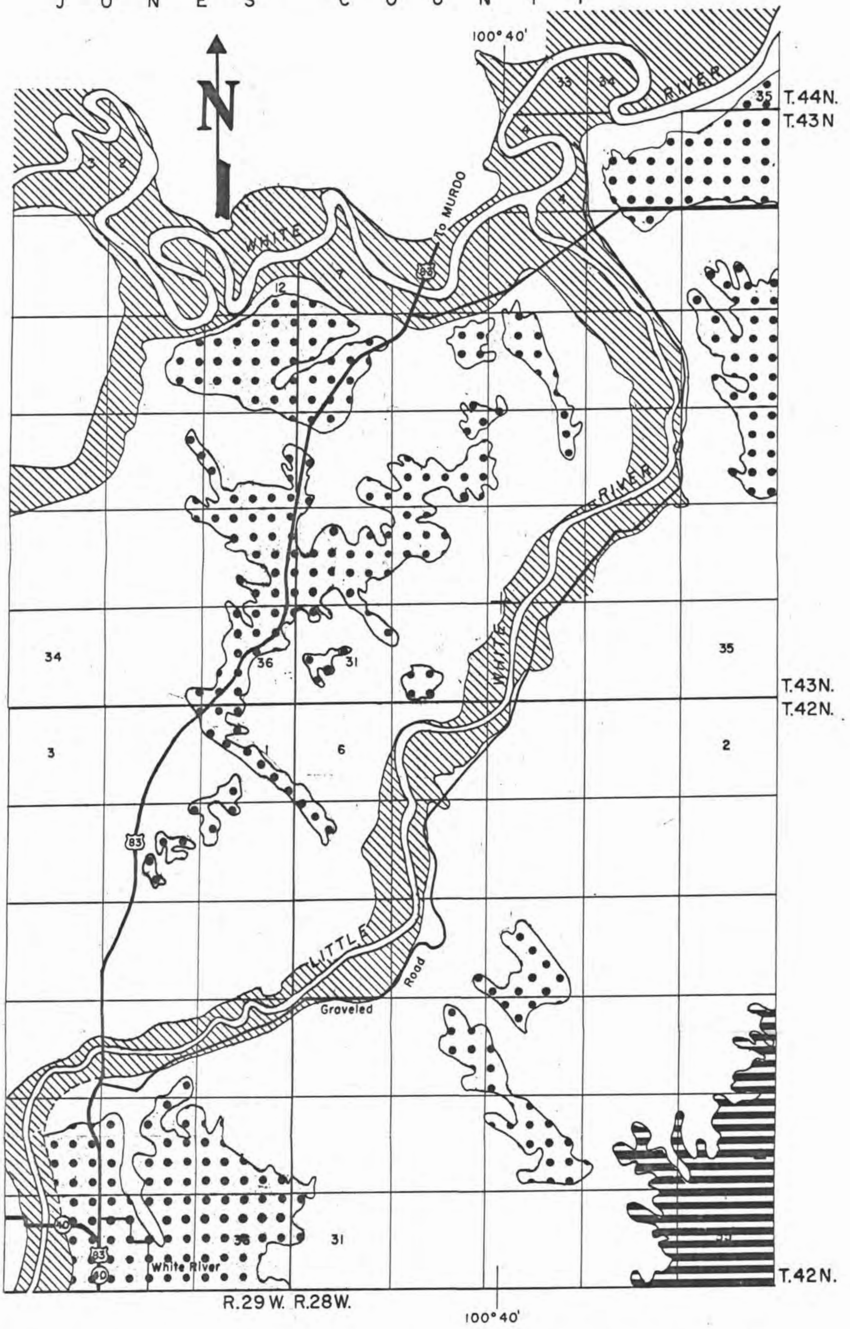
Figure 1. Generalized geologic map of the Little White River study area. (Modified from A. F. Agnew 1957)
